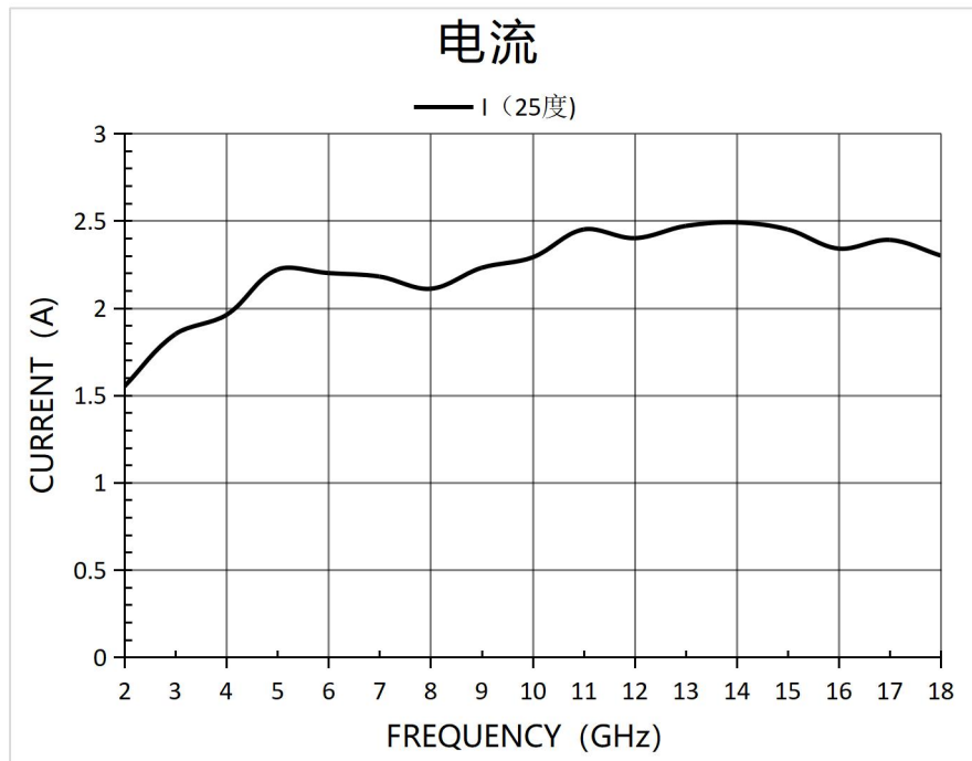
Current @ Pin=0dBm
