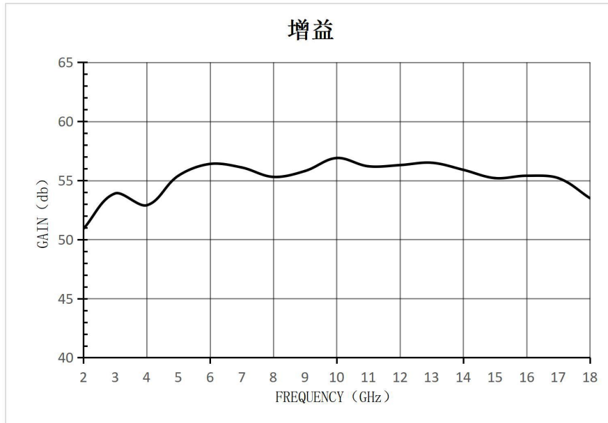
Gain @ Pin=-30dBm
