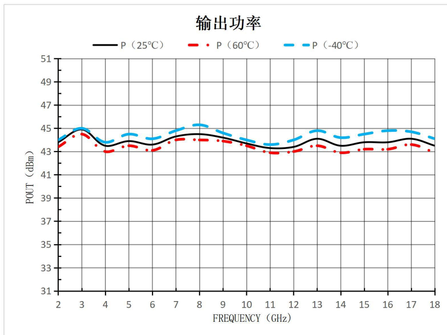
Output Power @ Pin=0dBm
