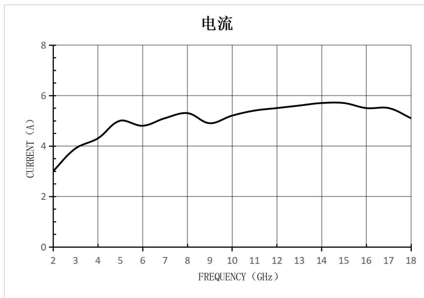
Current @ Pin=0dBm
